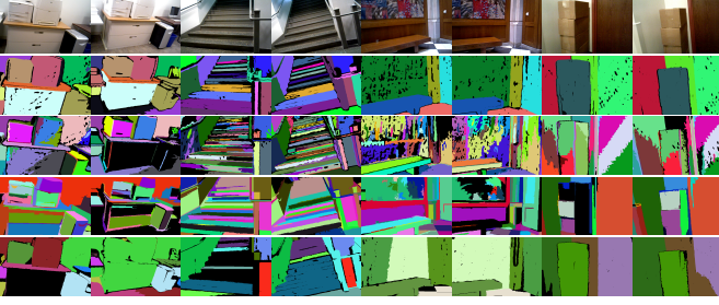
Figure 5. Comparison with bipartite matching on the ground truth dataset. Row 1: Source and target image pairs. Row 2: Matching results of the proposed method. Row 3-5: Matching results of bipartite matching on k -means superpixels (Row 3), superpixels using [16] (Row 4) and regions from [8] (Row 5).
