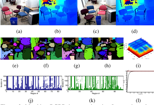
Figure 2. Matching RGBD image pair using Lagrangian relaxation. (a, b): Source color and depth image. (c, d): Target color and depth image. (e, f): Matching result from linear relaxation. (g, h): Matching result from the Lagrangian relaxation. (i): Matching cost matrix evolving during subgradient iteration. (j, k): x and y selection during iteration. A dot indicates a selection. (l): Energy of the Lagrangian dual during iteration.
