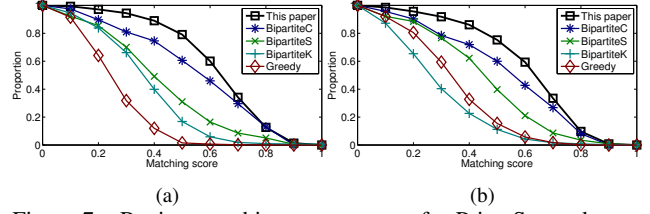
Figure 7. Region matching score curves for PrimeSense dataset (a) and NYU Kinect dataset (b). Proportions of tests with scores above different thresholds are shown. BipartiteC uses regions from [8], BipartiteS uses regions from [16] and BipartiteK uses regions from k -means.
