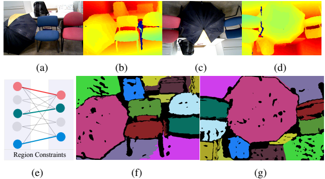
Figure 1. Finding region correspondence between RGBD images using bags of region candidates. We extract candidate regions using different methods to form bags of candidates on the source (a, b) and target (c, d) RGBD images. Our method optimizes the region selection and matching using the graph model in (e) and gives the matching result in (f, g). The same color in (f, g) indicates matched regions.
