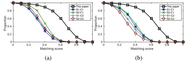
Figure 8. Comparison with hierarchical tree matching [3] on PrimeSense (a) and NYU Kinect (b) datasets. Proportions of tests with scores above different thresholds are shown. The tree method uses regions from two methods. In case one (C1), regions are from 3D normal k -means, and in case two (C2) regions are from [16]. For the tree method, two matching scores S1 and S2 are computed in each case.
