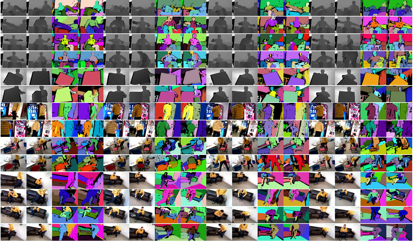
Figure 9. Sample results on more challenging dataset. These image pairs are extracted from five videos and images are 100 frames apart. These matching tests involve deformable and articulated human subjects, moving rigid objects, and occlusion between objects.
